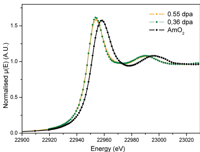
Figure 4. Am L_{II} normalized XANES spectra for the 0.36 and 0.55 dpa states and \text{Am}^{4+}\text{O}_2 reference sample.
