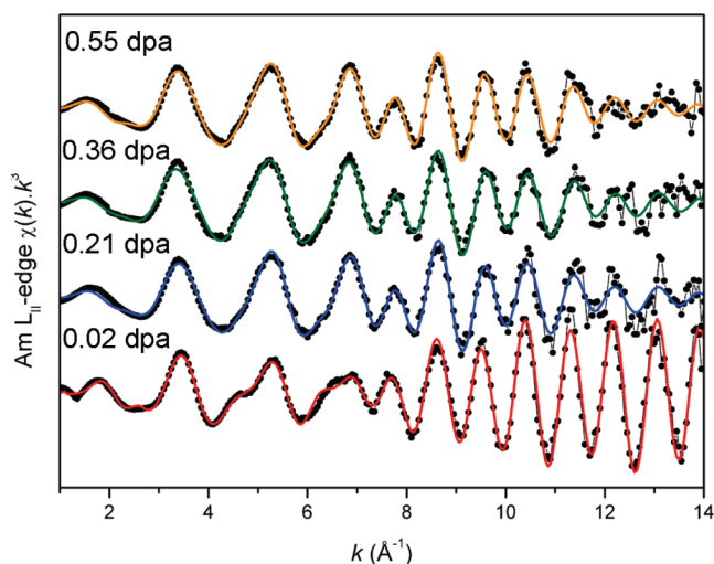
Figure 5. Am L_{II} -edge EXAFS spectra multiplied by k^3 for the 0.02, 0.21, 0.36, and 0.55 dpa states. Experimental data are displayed by symbols and fits by lines.
