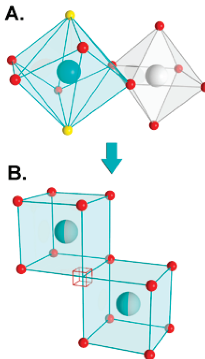
Figure 3. Coordination shells of Am and Zr cations in both structures. In the pyrochlore structure (A), Am (blue) is surrounded by two short-distance \text{O}(8b) atoms (yellow) and six longer-distance \text{O}(48f) atoms (red). Zr (gray) is surrounded by six equidistant \text{O}(48f) 's. In the defect-fluorite structure (B), both Am and Zr share the same crystallographic site, and O anions occupy 7/8 of a unique site.
